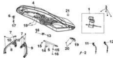
F17 FUEL TANK
